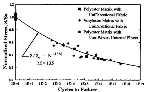
b. Unidirectional Fiberglass Composite.
