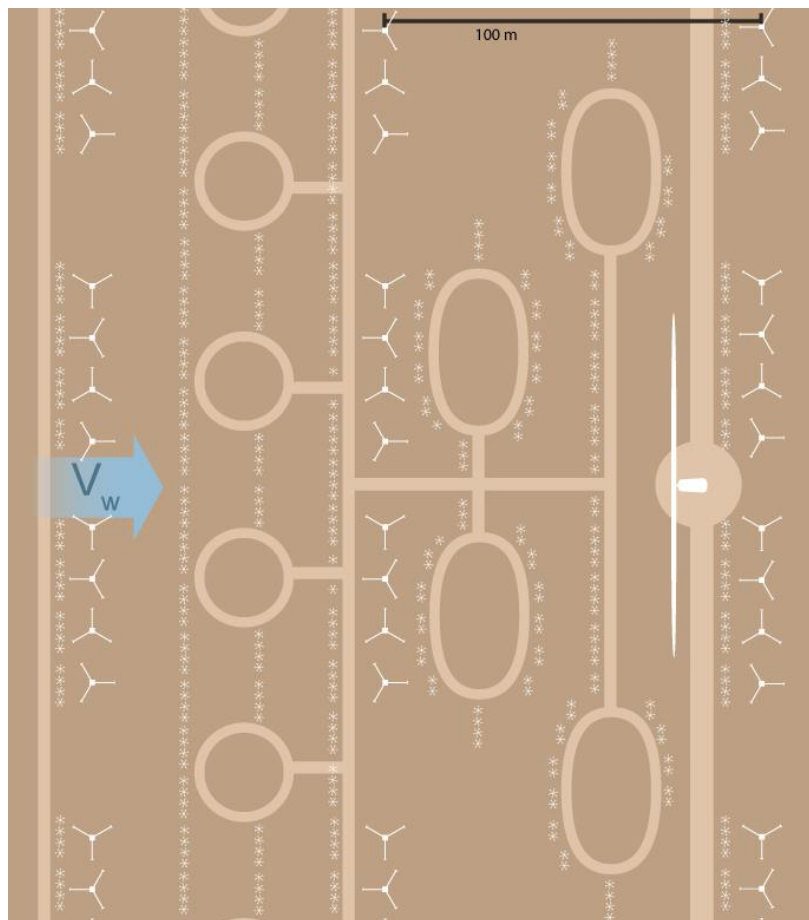
Figure 3 This 250 X 250 sq. meter slice of the Calabazon wind farm in Figure 1 shows one way in which VAWTs of different heights could be placed around a newly installed 2 MW HAWT on a 65m tower. In this graphical representation, there are 428 of the 3kW VAWTs and 39 of the WHI's 70kW VAWTs and one 2 MW HAWT.
